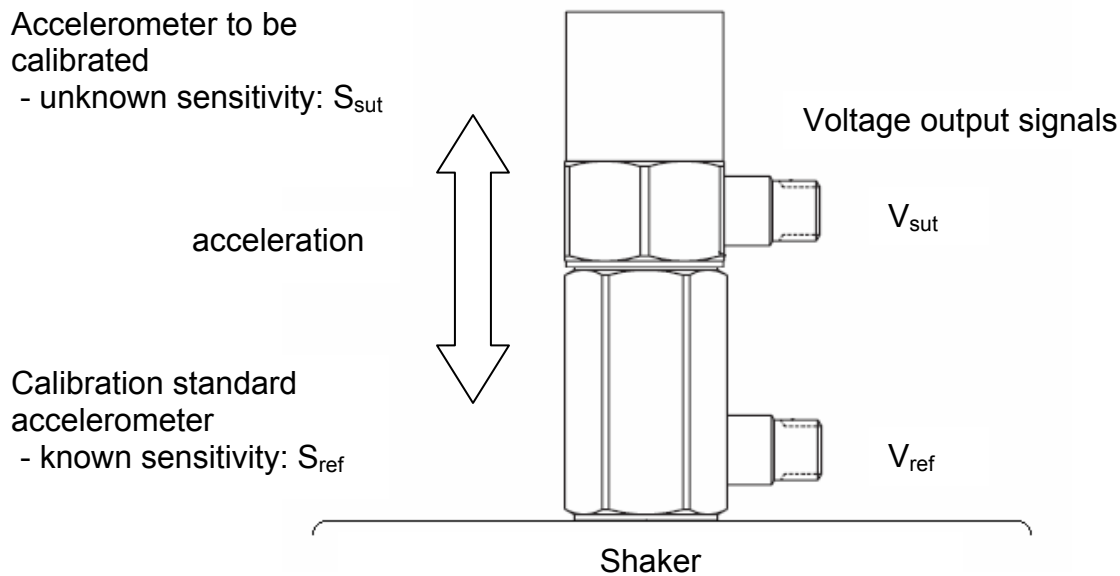
Figure 1: Back-to-back technique
