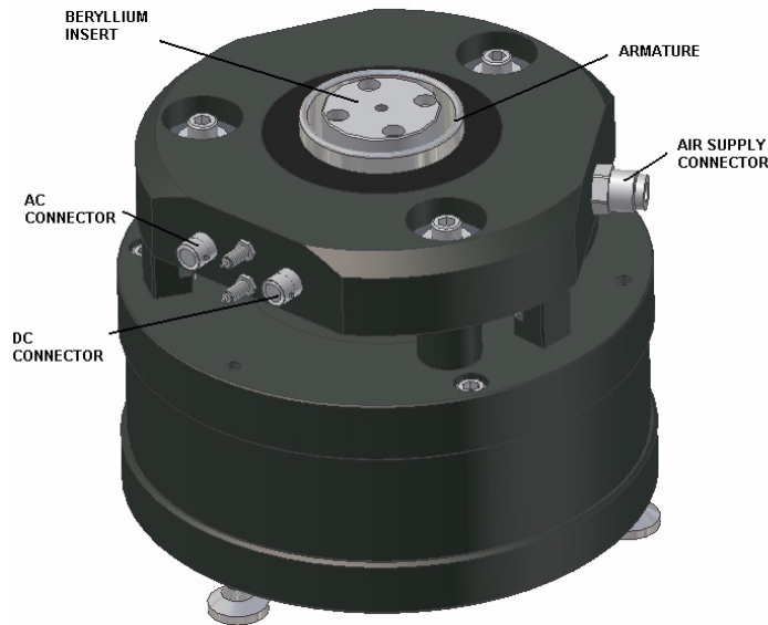
Figure 3: Air bearing shaker [3]
