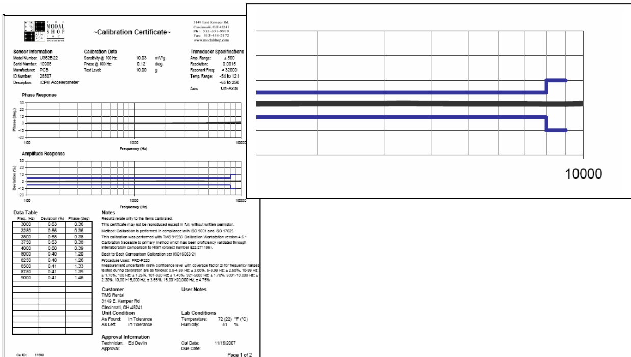
Figure 10. Calibration certificate generated using precision air-bearing calibration shaker. Notice the complete absence of transverse motion induced glitches around 3500 and 9000 Hz.
