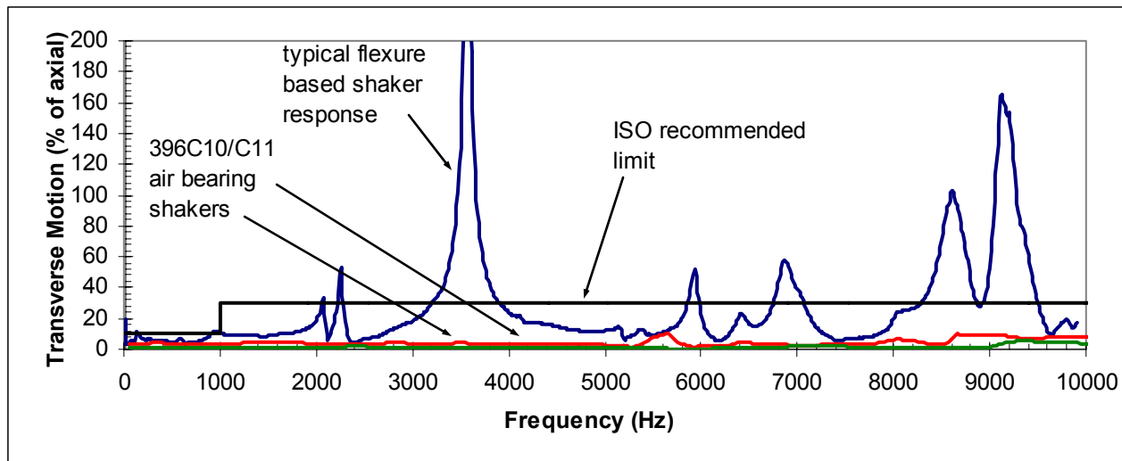
Figure 3. Transverse motion measured on flexure-based and air-bearing calibration shakers, plotted against ISO 16063-21 recommended limits
