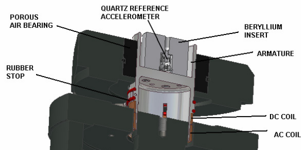
Figure 4: Cross section view of the air bearing shaker [3]
