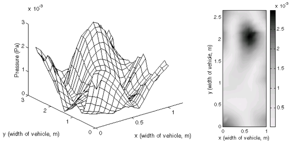
Figure 8: 3-d mesh and gray-scale map of the pressure magnitude measured at 72 mm above the floor pan.
