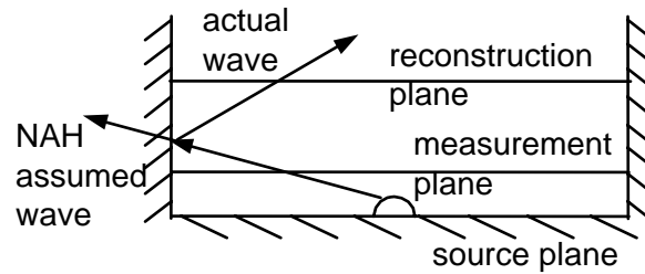
Figure 3: Illustration of a wall reflection.
