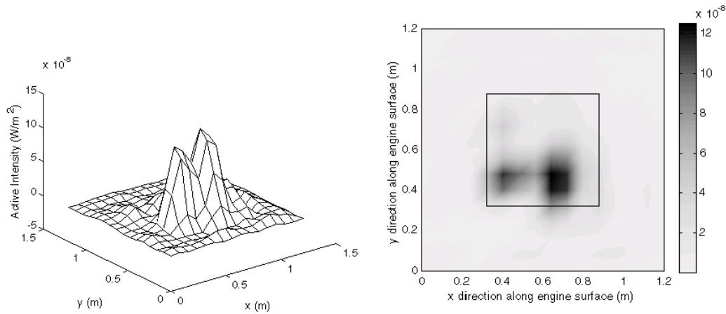
Figure 11: 3-d mesh and gray-scale map of the active intensity projected onto the engine surface.
