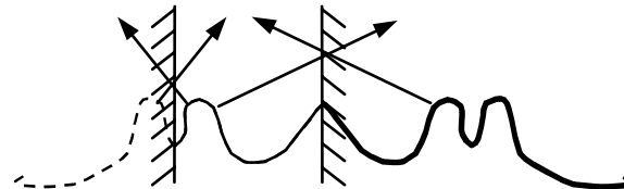
Figure 4: Illustration of wall model created by extending the measured pressure distribution. Solid line – measured pressure. Dotted line – mirror image. Thick line – infinite periodic extension.
