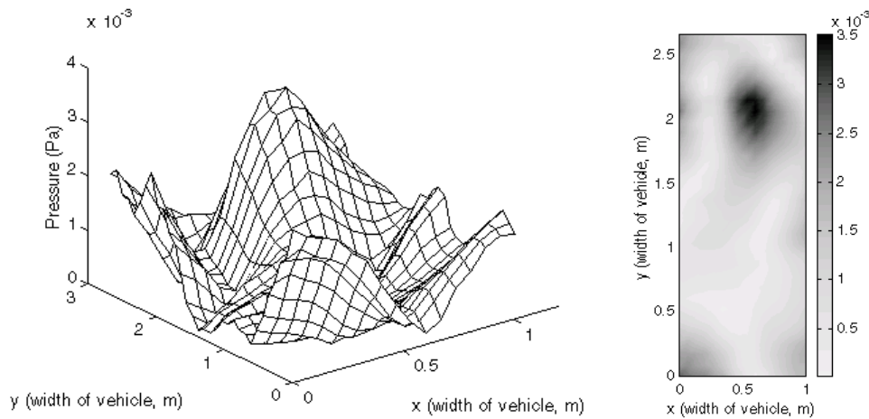
Figure 7: 3-d mesh and gray-scale map of the pressure magnitude measured at 22 mm above the floor pan.
