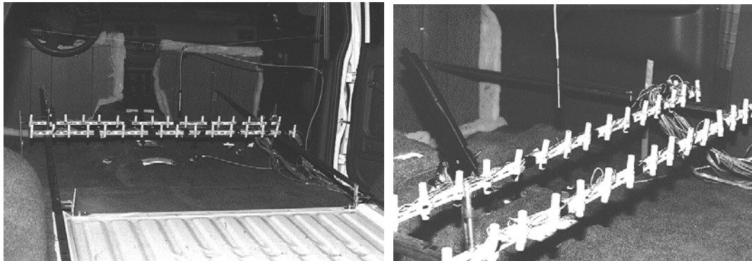
Figure 6: Grid setup of microphone array for interior vehicle cabin test.
