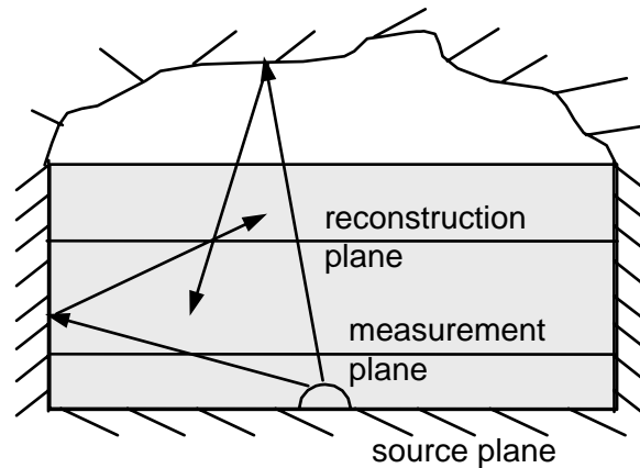
Figure 5: Illustration of the valid regions of reconstructions for a full enclosure under the assumptions outlined in this section.
