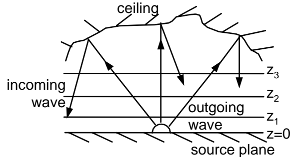
Figure 2: Illustration of ceiling reflections.
