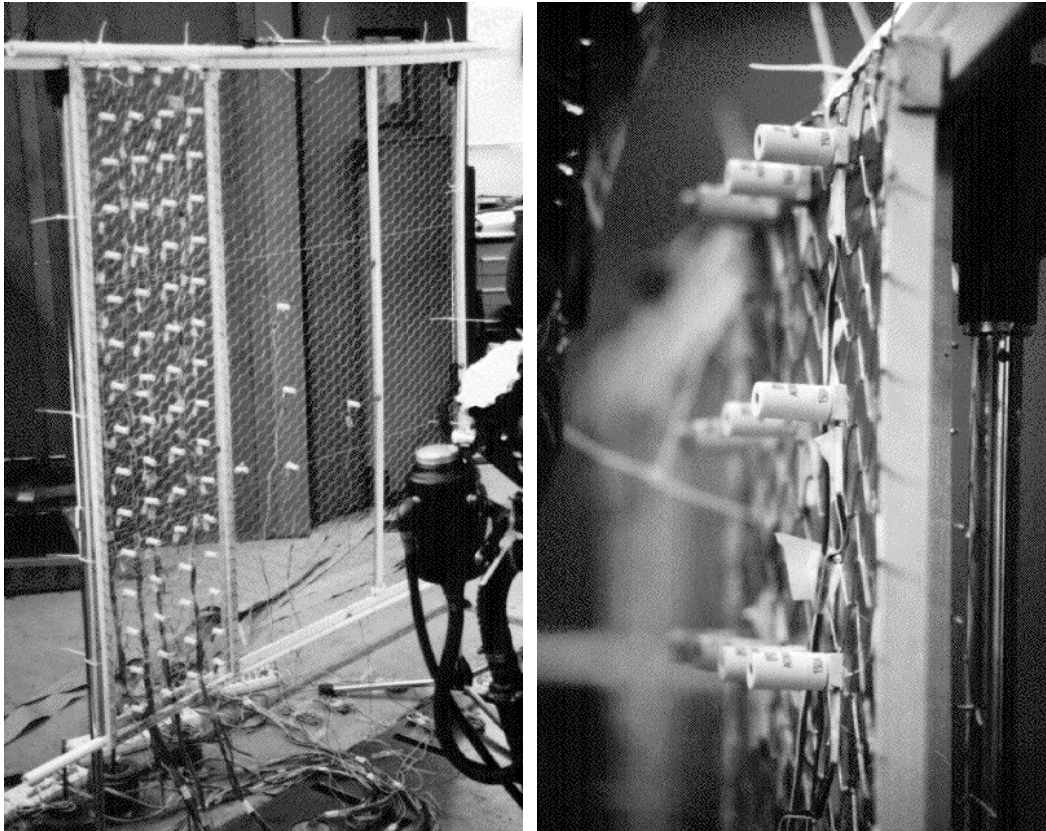
Figure 10: Grid setup of microphone array for idling engine test.
