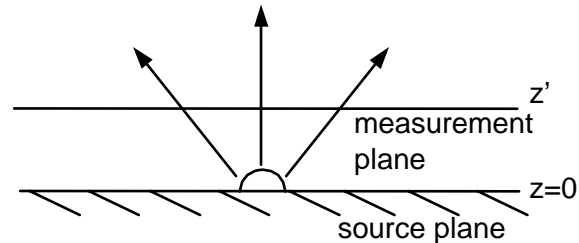
Figure 1: Illustration of free-field NAH in a planar geometry.
